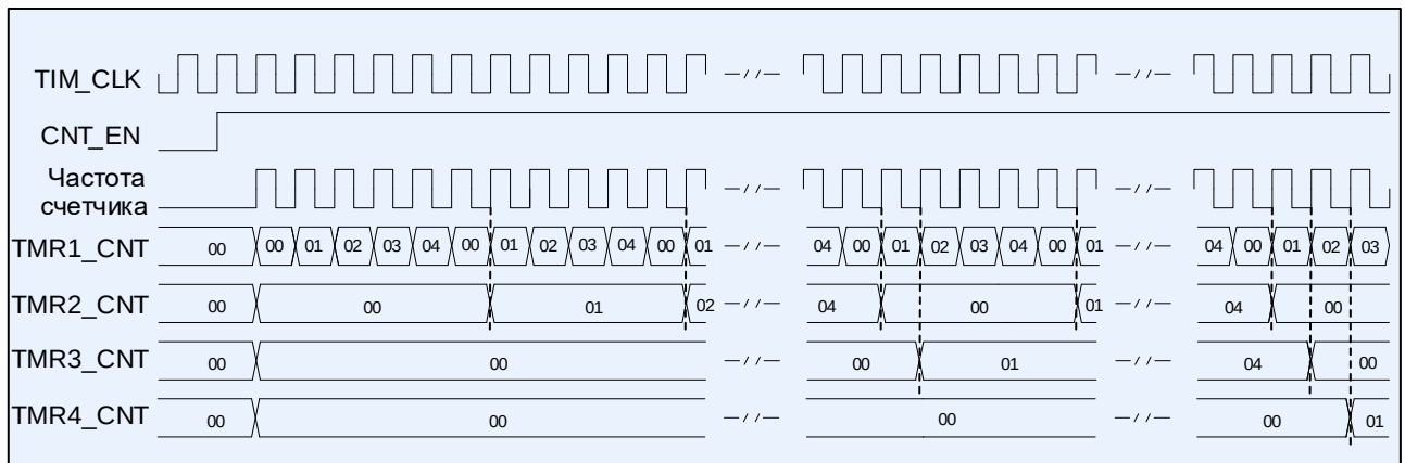
Рисунок 56 – Диаграммы работы четырех таймеров в каскаде TIMER1: DIR = 0, EVNT_SEL[3:0] = 0000, CNT_MODE[1:0] = 00; TIMER2: DIR = 0, EVNT_SEL[3:0] = 0001, CNT_MODE[1:0] = 10; TIMER3: DIR = 0, EVNT_SEL[3:0] = 0010, CNT_MODE[1:0] = 10; TIMER4: DIR = 0, EVNT_SEL[3:0] = 0011, CNT_MODE[1:0] = 10.
